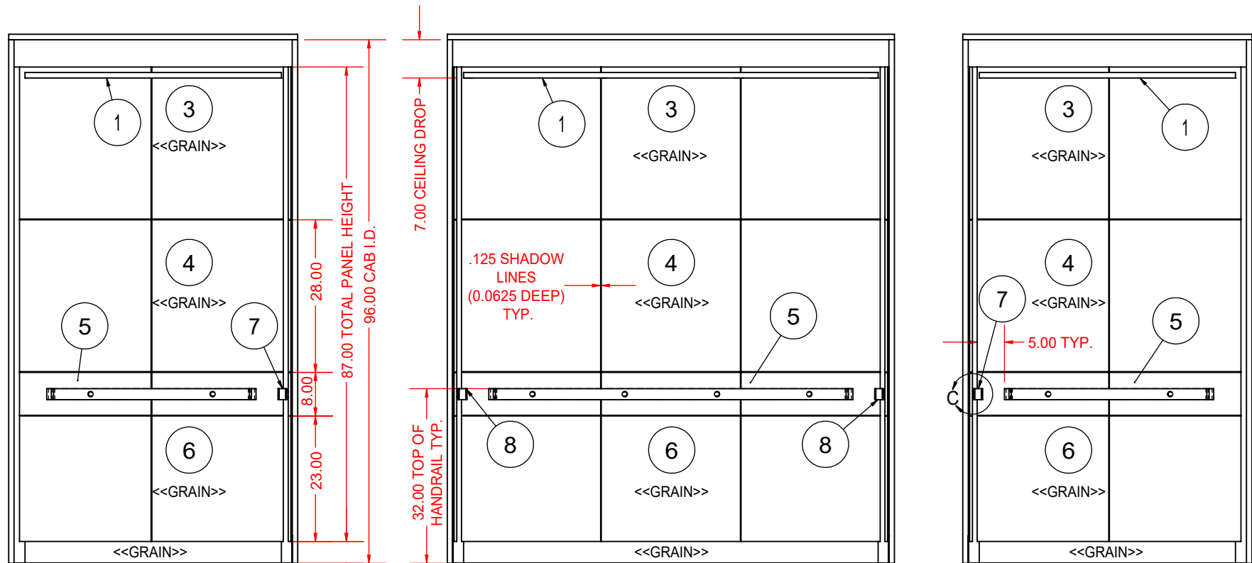
WALL ELEVATION A
